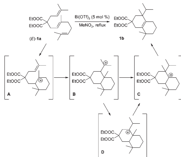
Scheme 1. Double Cyclization of ( E )- 1a Catalyzed by Bi(OTf) 3
